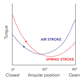
Symmetric yoke mechanism Spring to open
